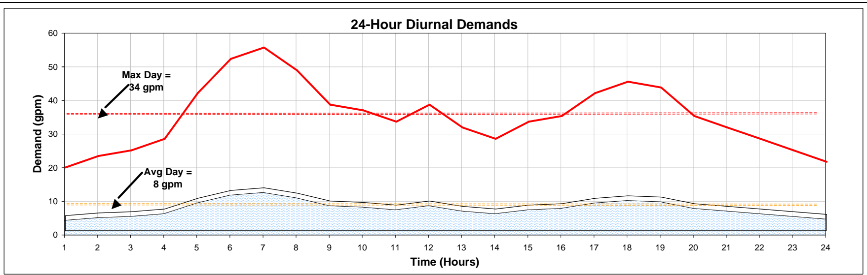
FIGURE 11 DORENA CLUSTER DAILY DIURNAL DEMAND PATTERNS
